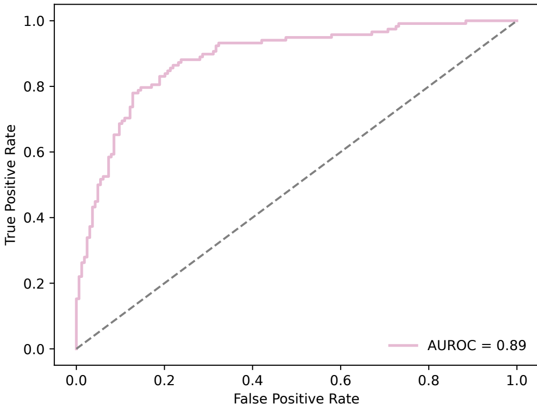
MLP ROC Curve
